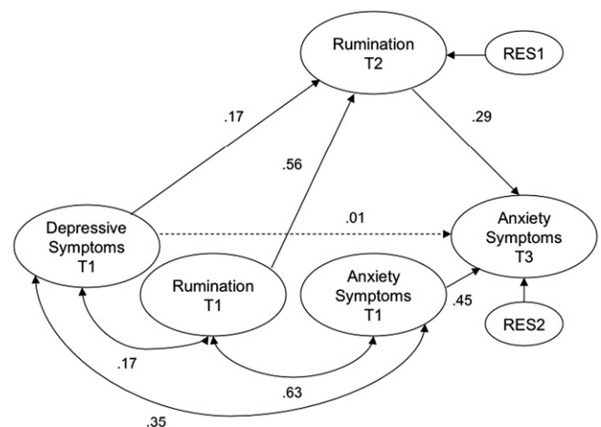
Fig. 1. Note. Figure represents the longitudinal mediation model in adolescents. Numbers represent standardized path coefficients ( \beta ). All paths shown are significant ( p < .05 ), except those drawn with broken lines. All constructs were modeled as latent variables. Due to space constraints, indicator variables are not displayed.
